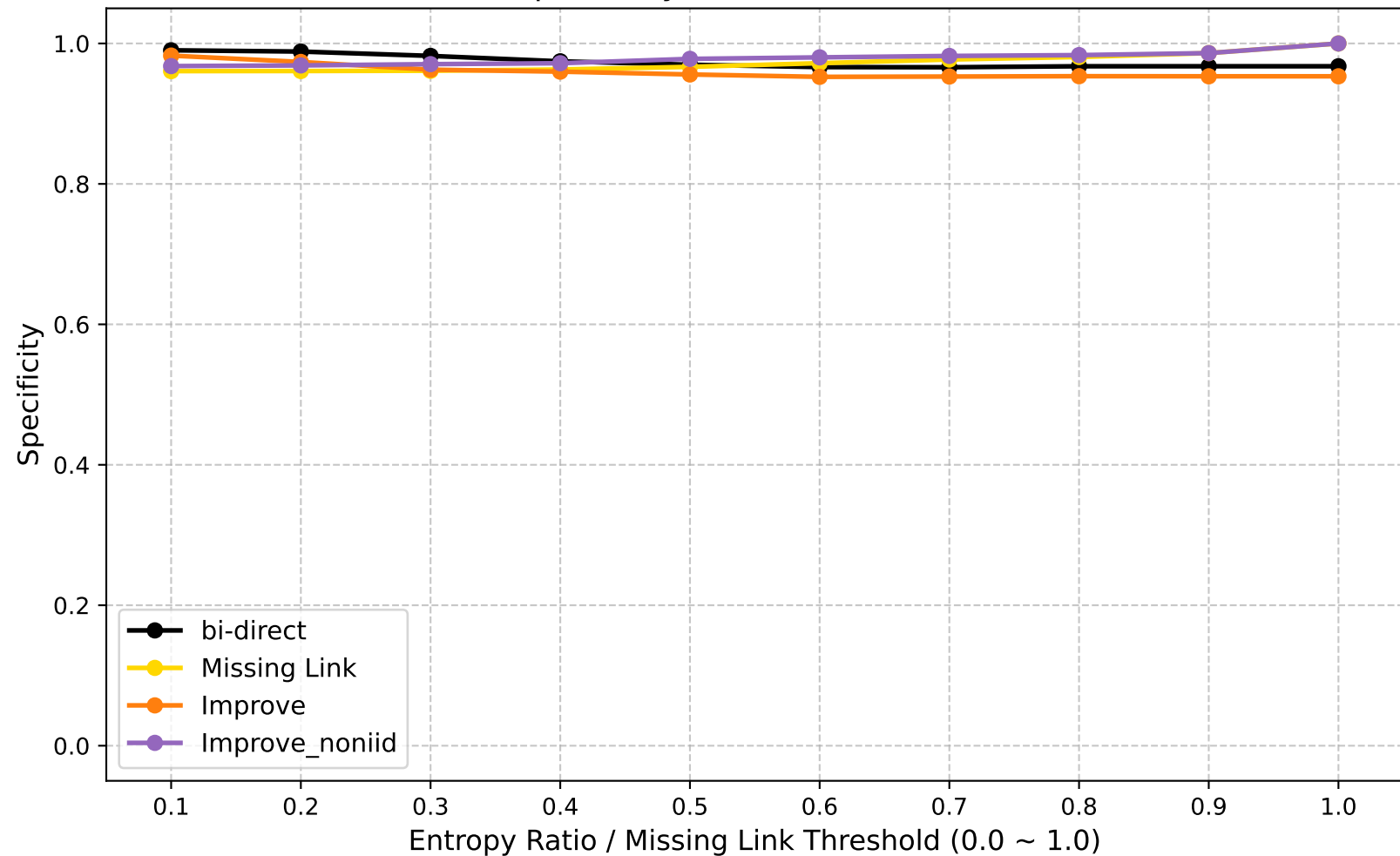
Specificity (Global Round: 15)
