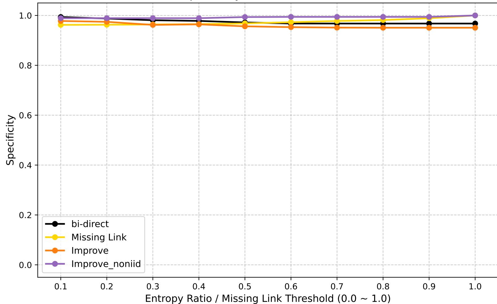
Specificity (Global Round: 20)
