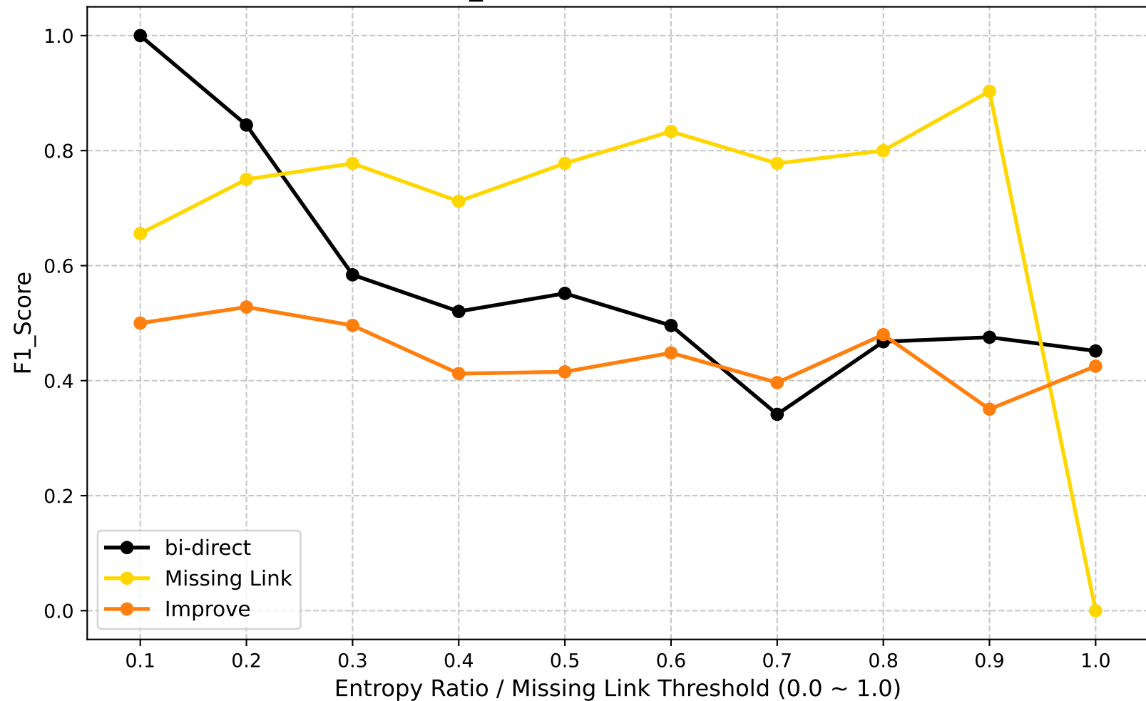
F1_Score (Global Round: 5)
