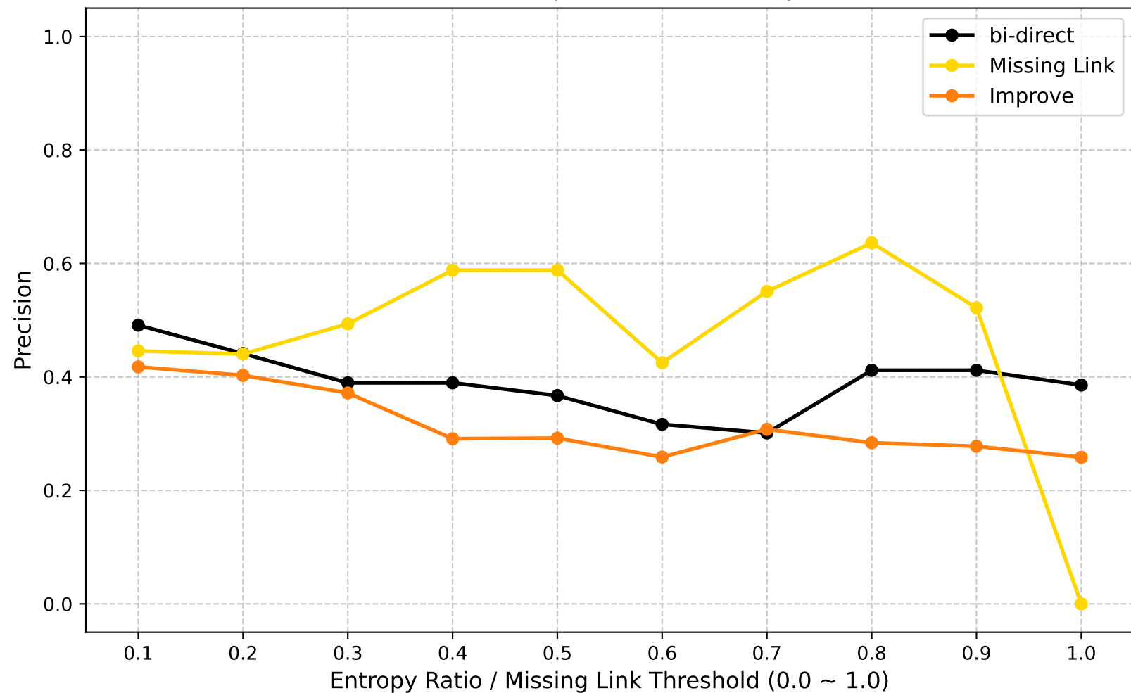
Precision (Global Round: 10)
