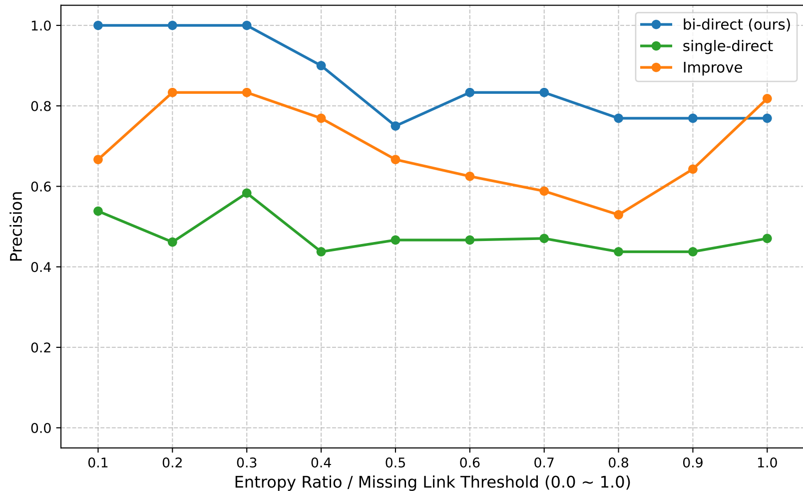
Precision (Global Round: 5)
