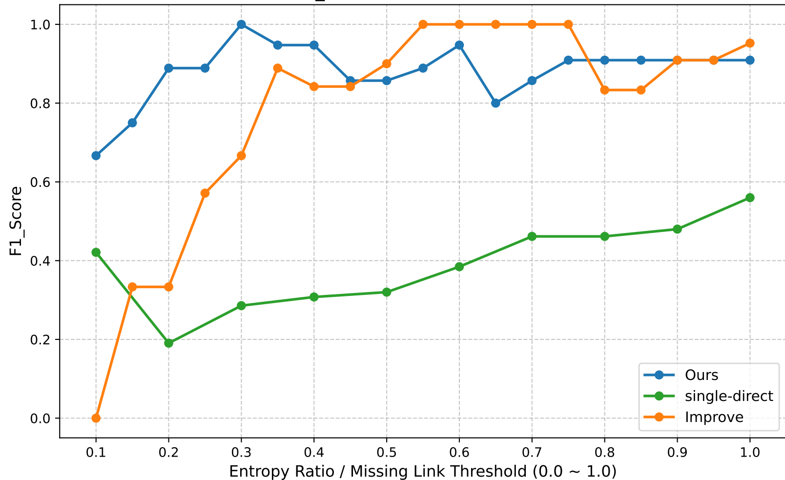
F1_Score (Global Round: 15)
