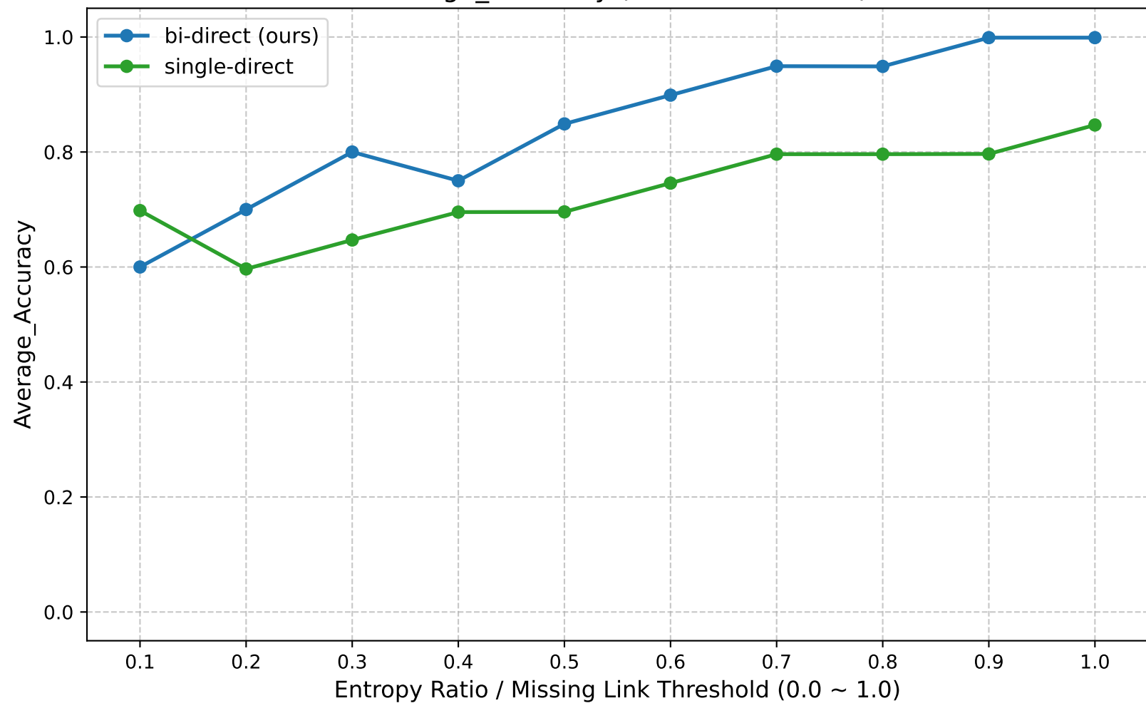
Average_Accuracy (Global Round: 15)
