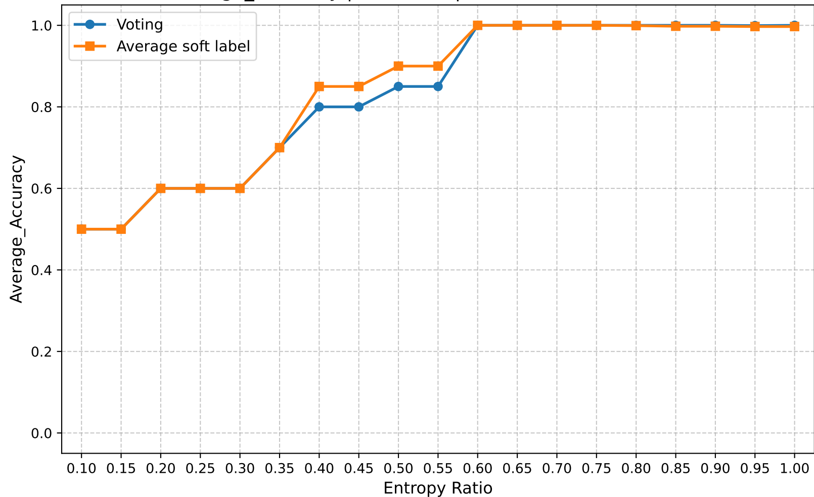
Average_Accuracy | Round 10 | Confuse Model Ratio 0.30
