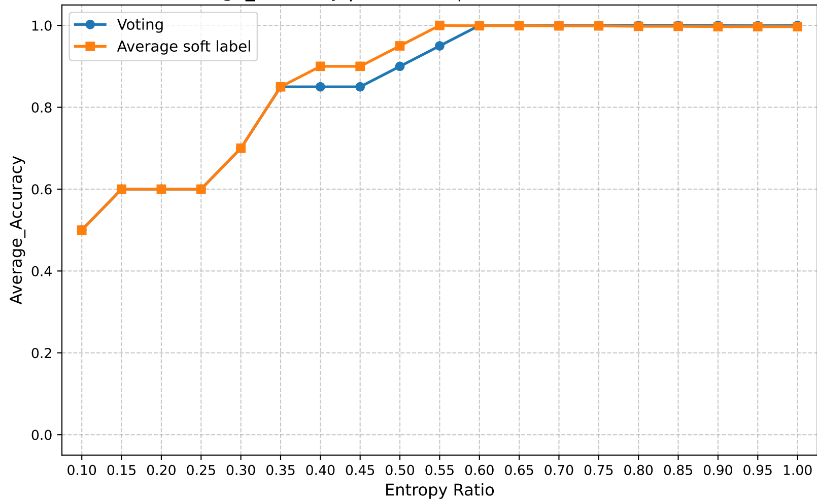
Average_Accuracy | Round 10 | Confuse Model Ratio 0.40
