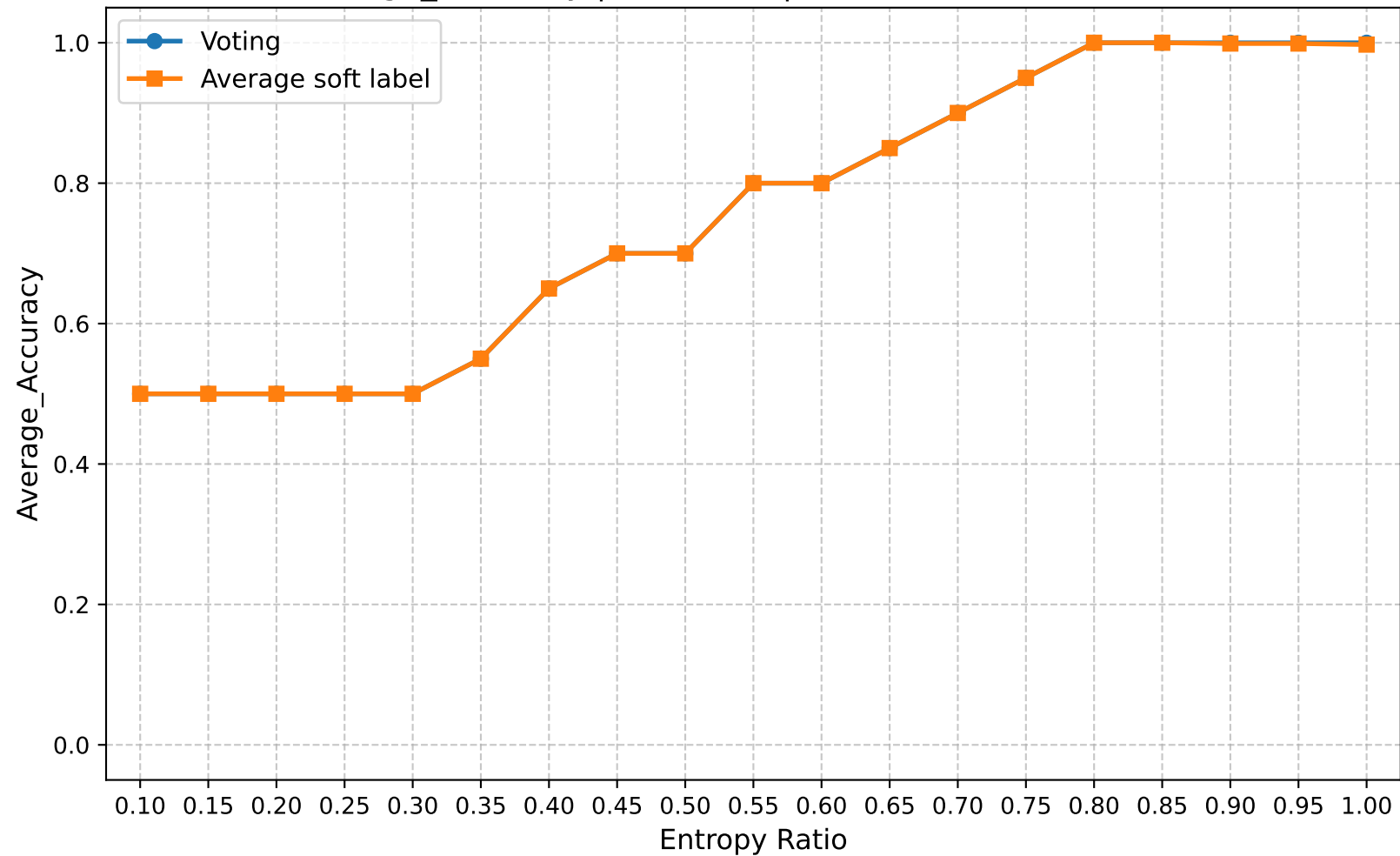
Average_Accuracy | Round 20 | Confuse Model Ratio 0.10
