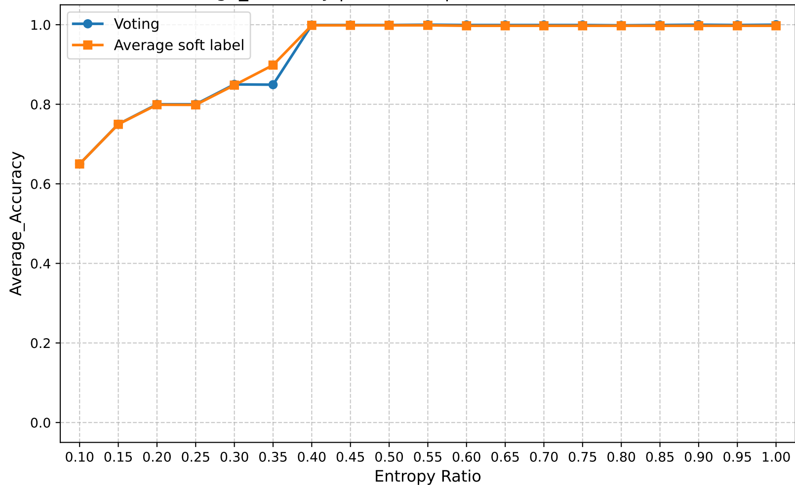
Average_Accuracy | Round 20 | Confuse Model Ratio 0.80
