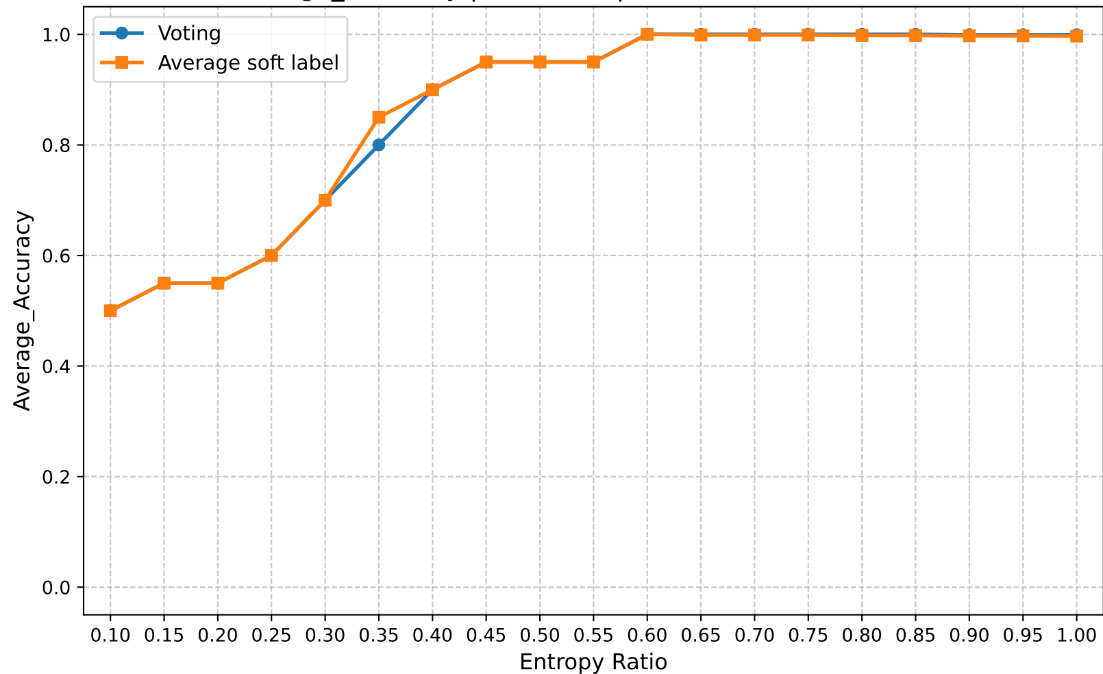
Average_Accuracy | Round 25 | Confuse Model Ratio 0.40
