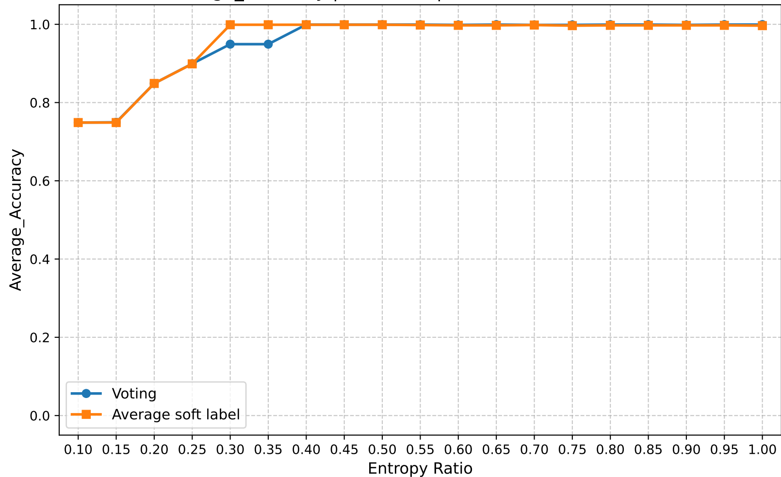
Average_Accuracy | Round 25 | Confuse Model Ratio 0.90
