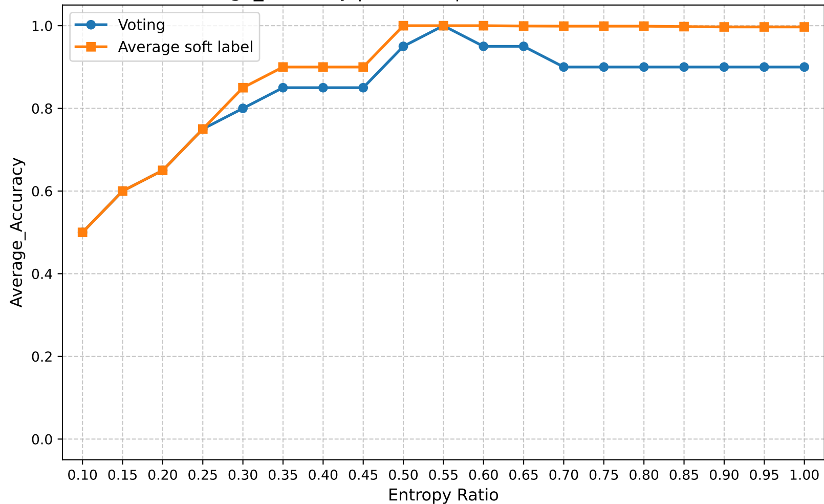
Average_Accuracy | Round 5 | Confuse Model Ratio 0.40
