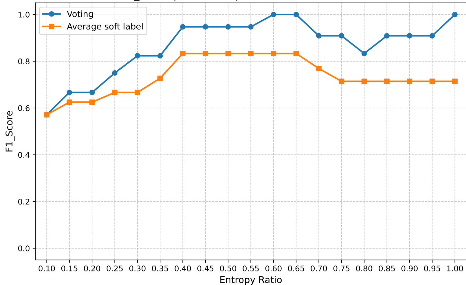
F1_Score | Round 10 | Confuse Model Ratio 0.70
