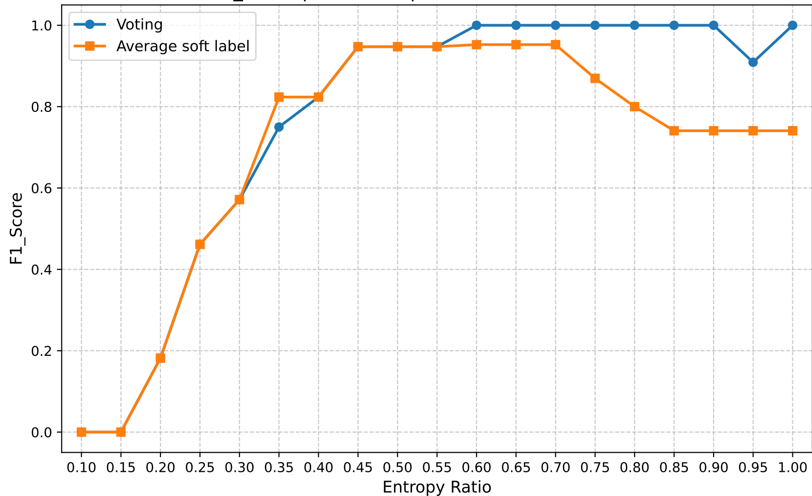
F1_Score | Round 20 | Confuse Model Ratio 0.40
