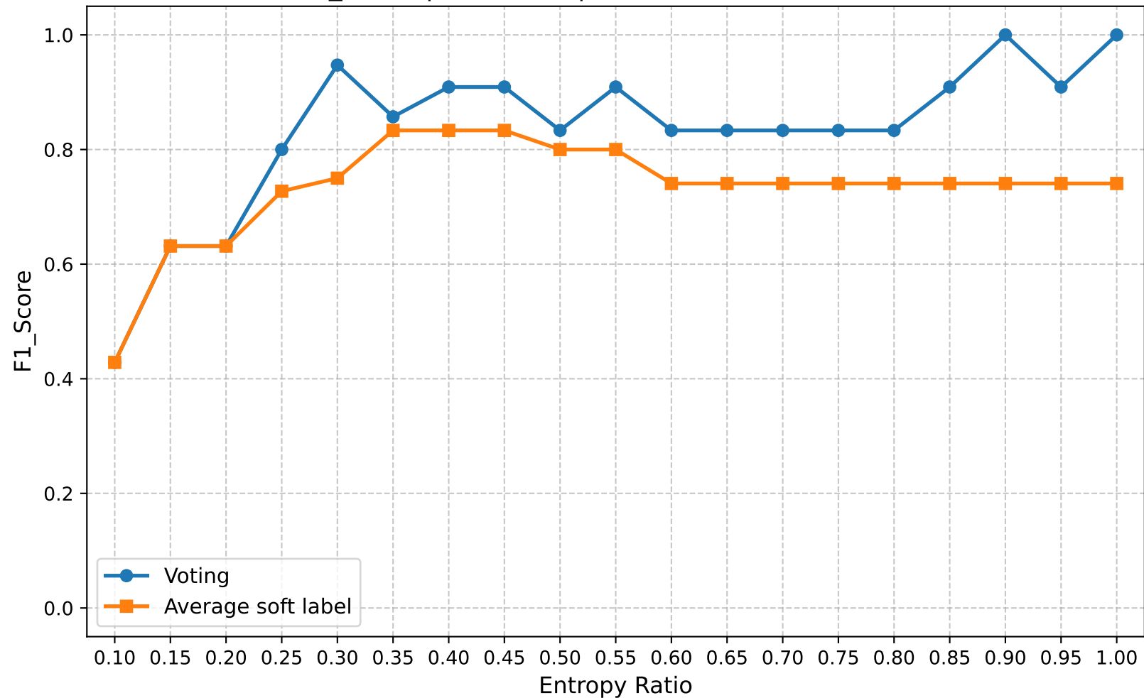
F1_Score | Round 20 | Confuse Model Ratio 1.00
