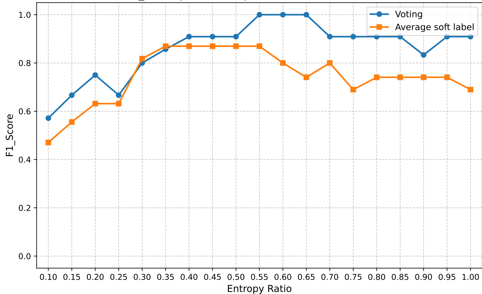
F1_Score | Round 25 | Confuse Model Ratio 0.80
