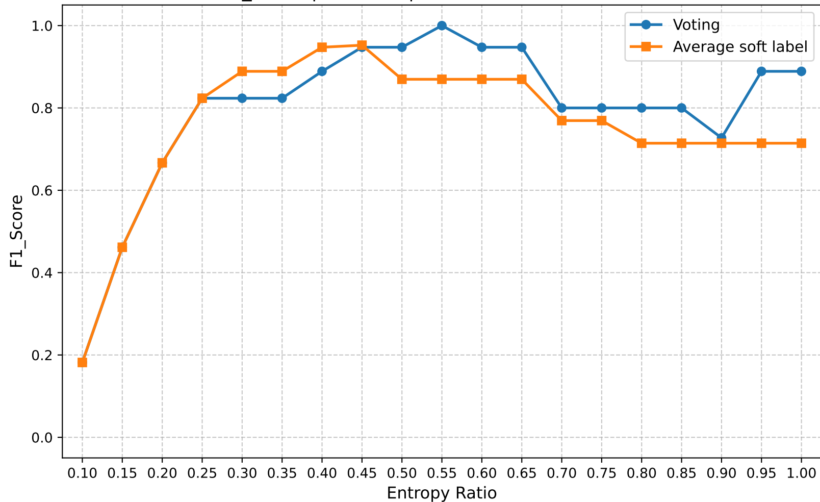
F1_Score | Round 5 | Confuse Model Ratio 0.60
