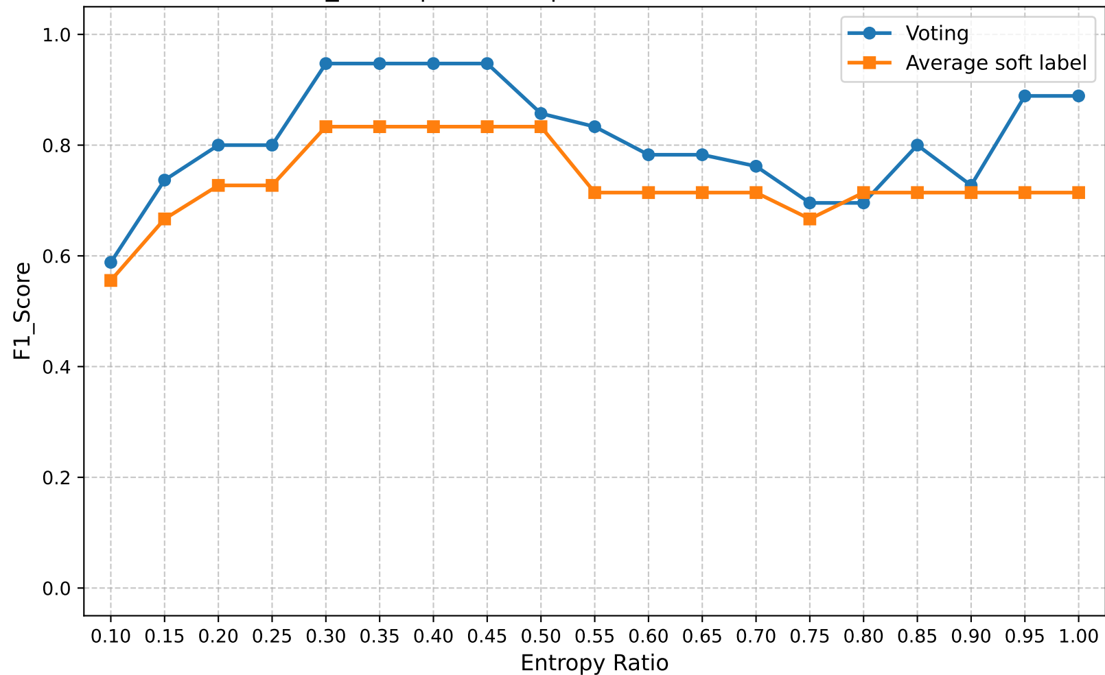
F1_Score | Round 5 | Confuse Model Ratio 1.00
