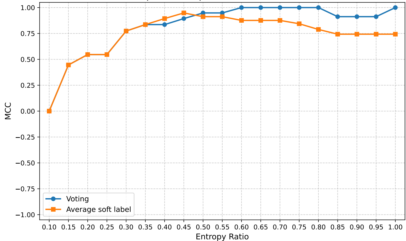
MCC | Round 10 | Confuse Model Ratio 0.50
