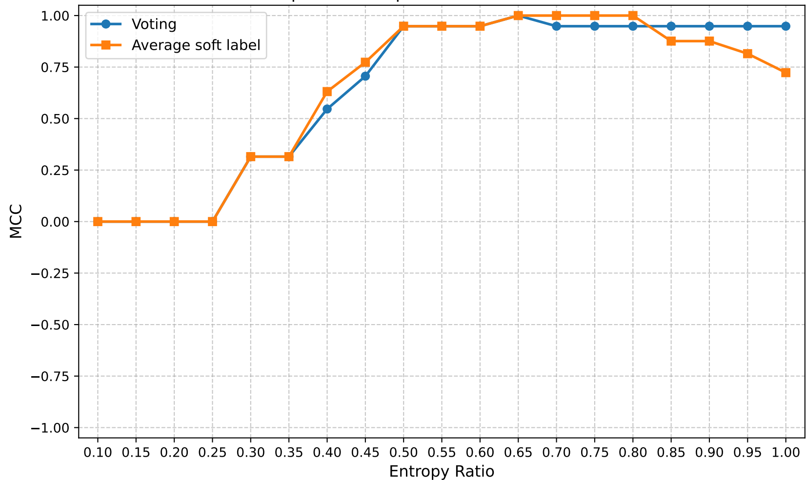
MCC | Round 15 | Confuse Model Ratio 0.20
