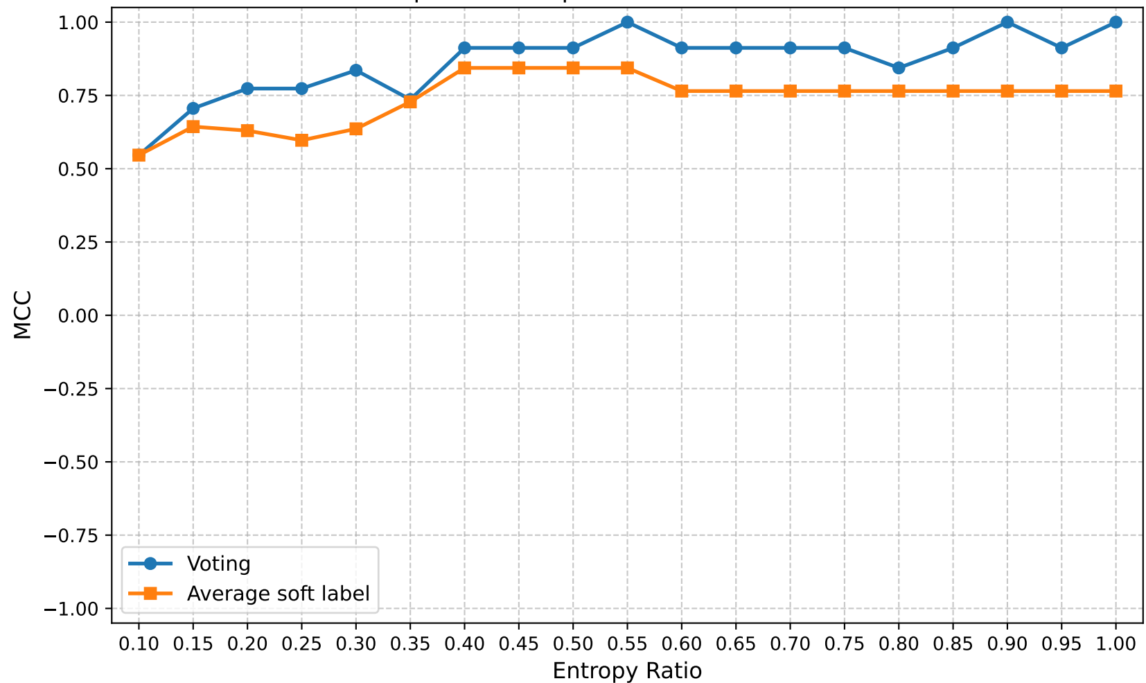
MCC | Round 20 | Confuse Model Ratio 0.80
