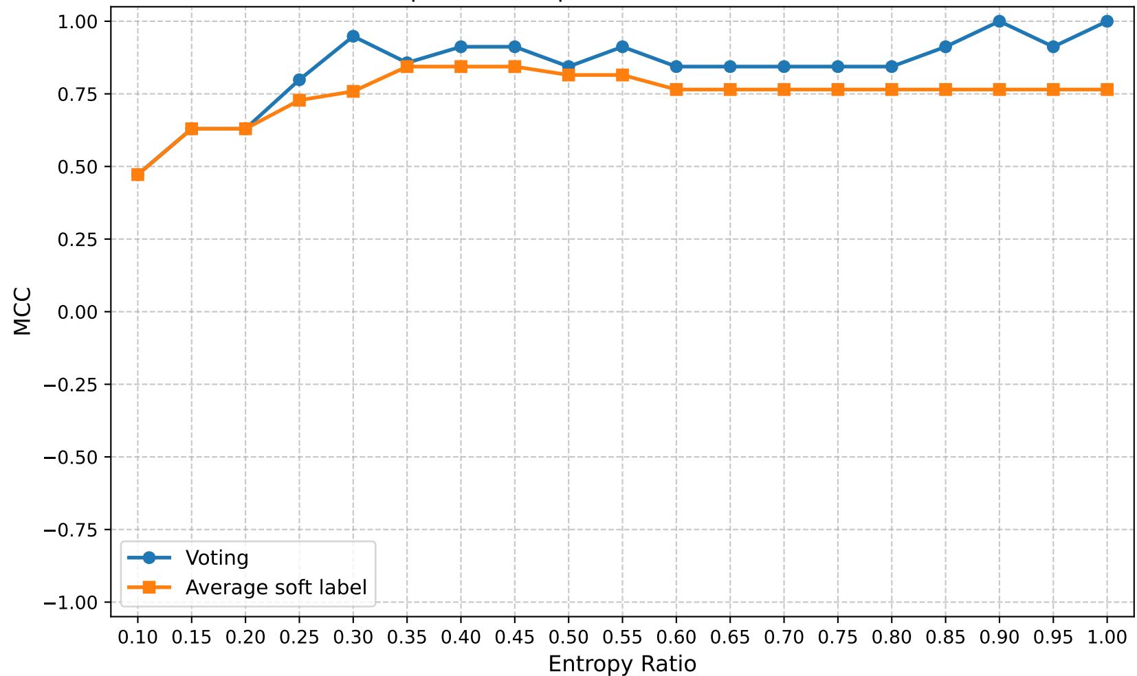
MCC | Round 20 | Confuse Model Ratio 1.00
