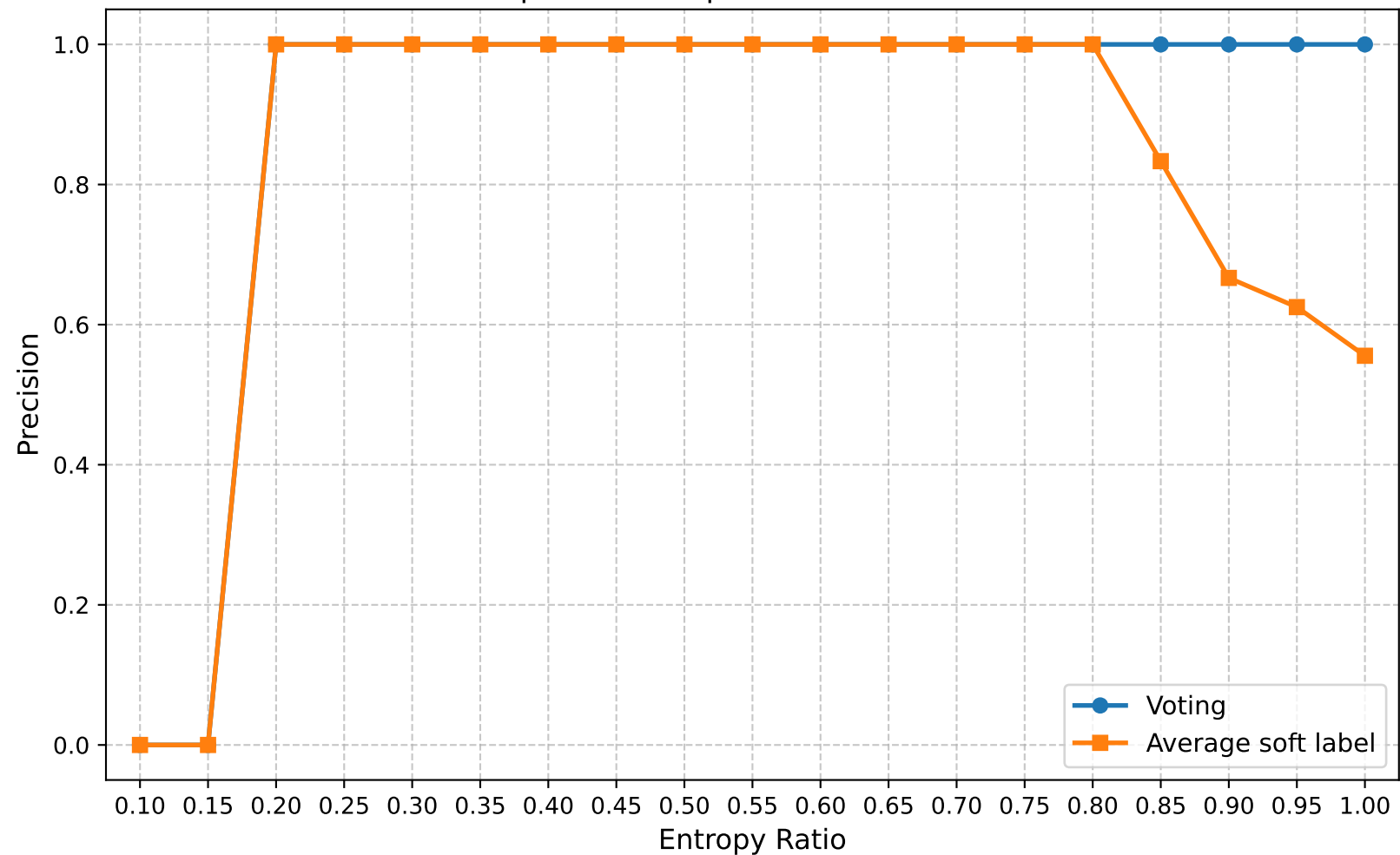
Precision | Round 10 | Confuse Model Ratio 0.20
