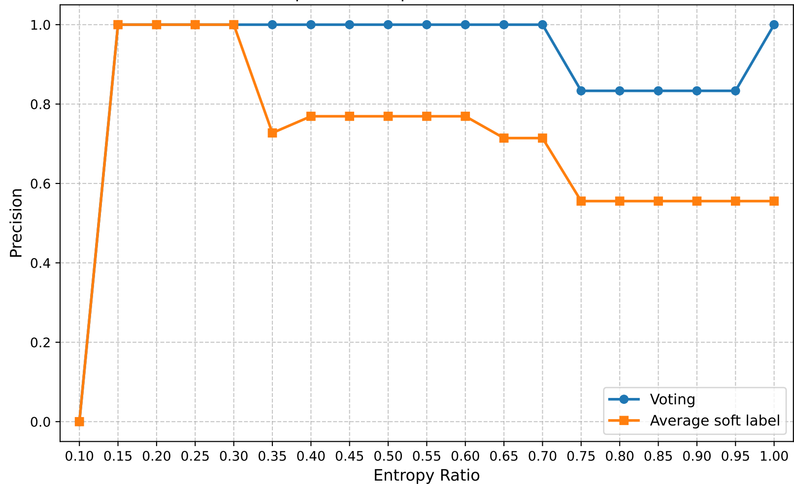
Precision | Round 10 | Confuse Model Ratio 0.60
