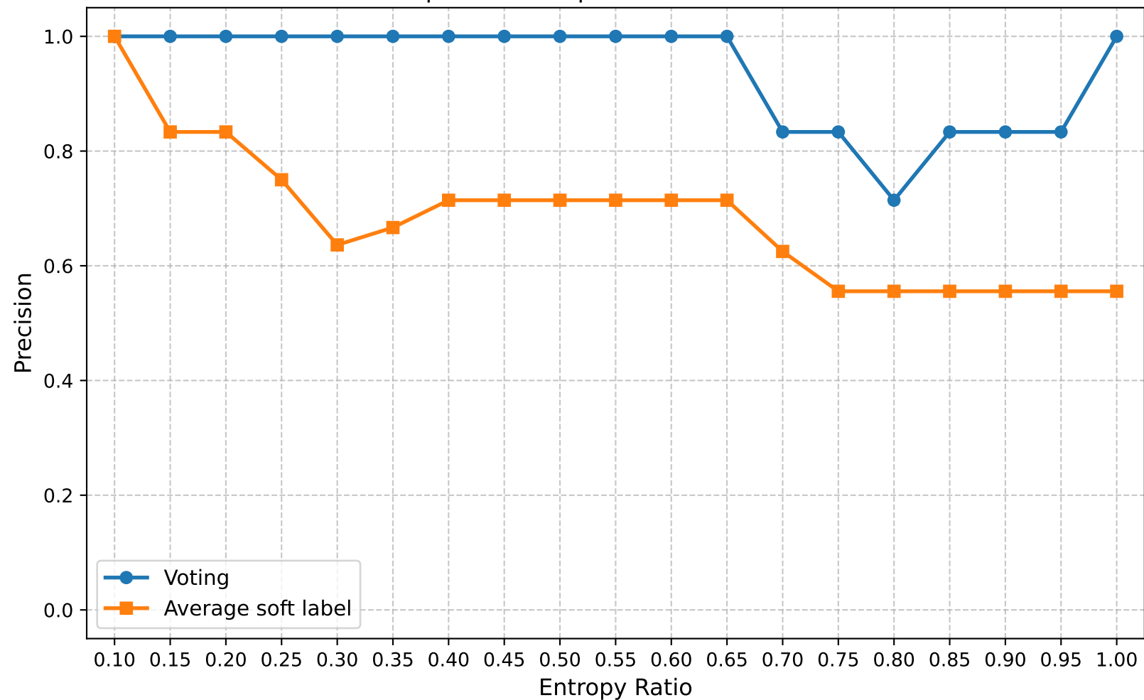
Precision | Round 10 | Confuse Model Ratio 0.70
