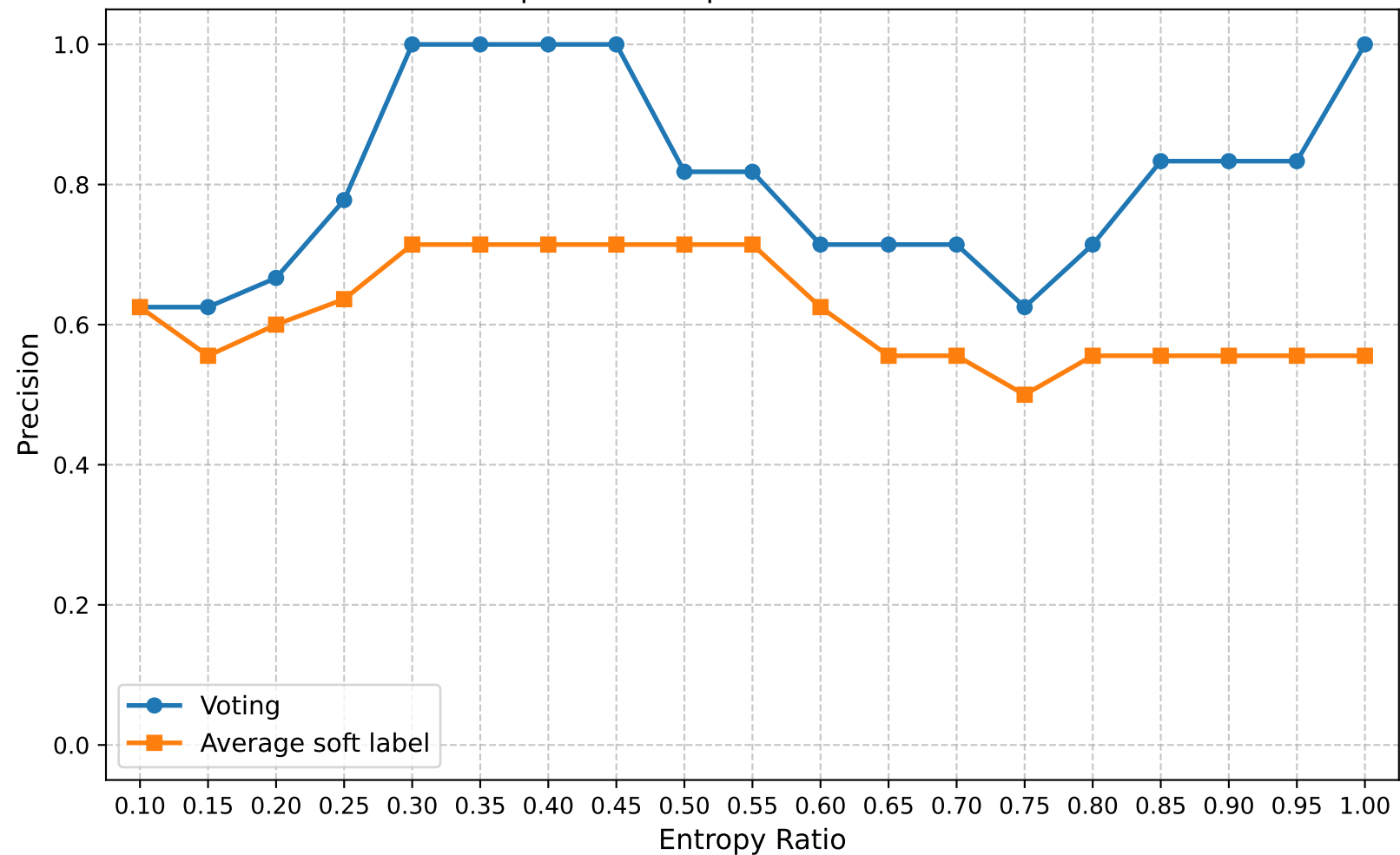
Precision | Round 10 | Confuse Model Ratio 0.90
