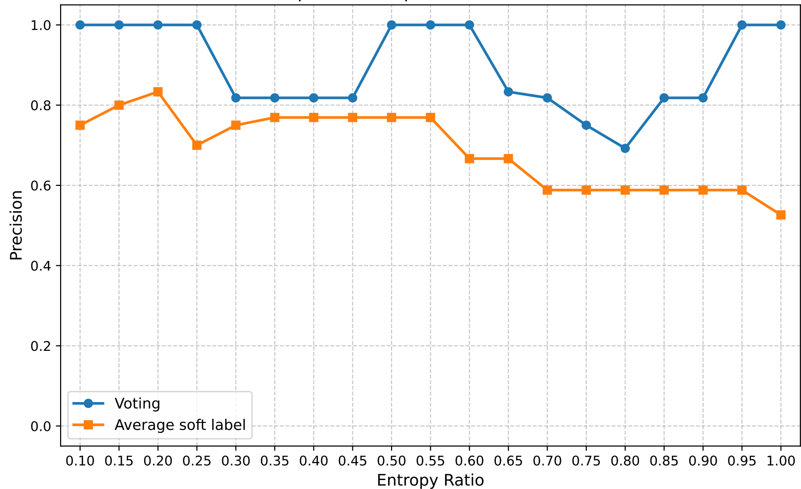
Precision | Round 15 | Confuse Model Ratio 0.80
