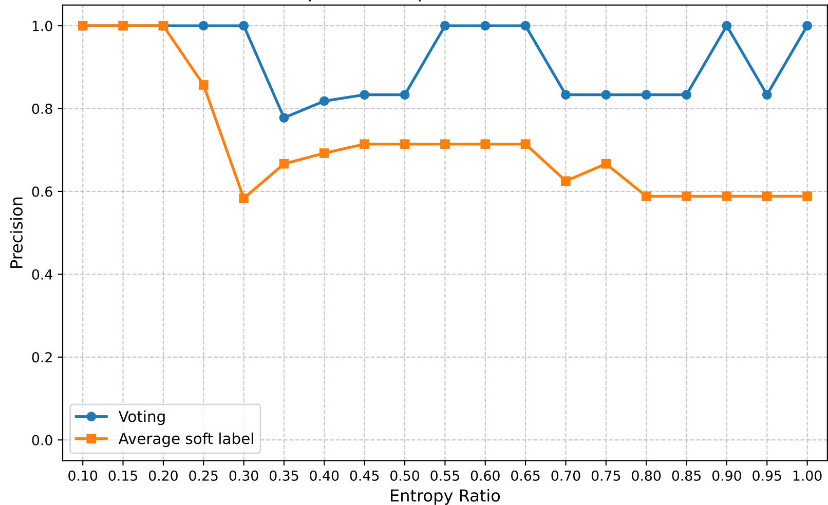
Precision | Round 20 | Confuse Model Ratio 0.70
