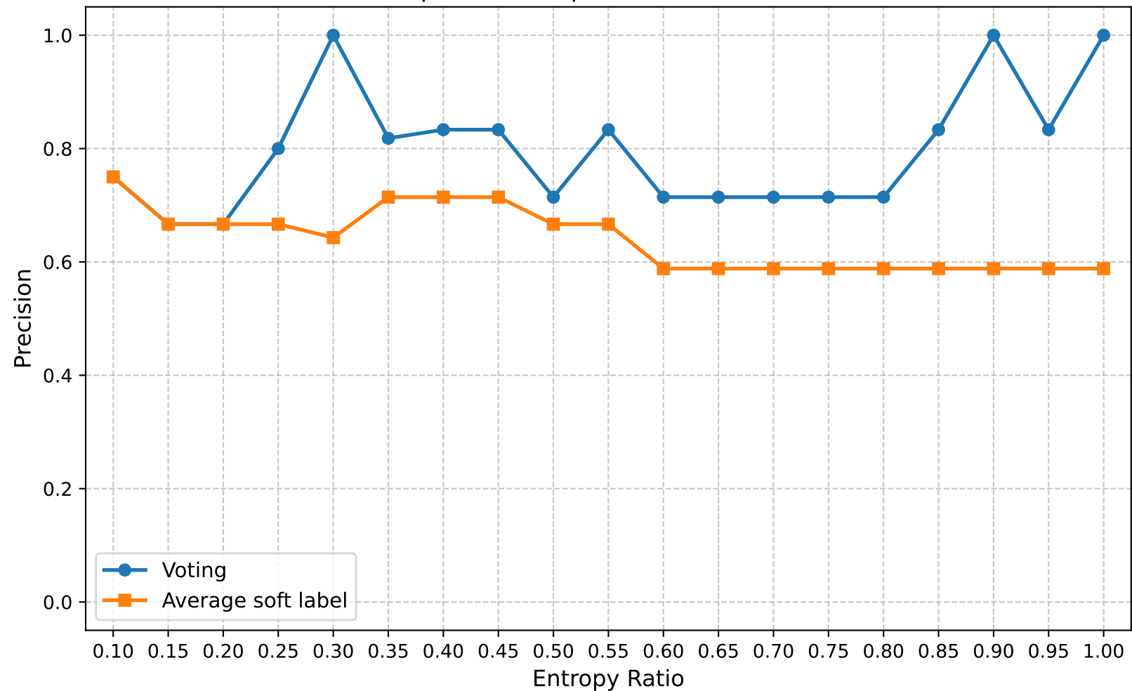
Precision | Round 20 | Confuse Model Ratio 0.90
