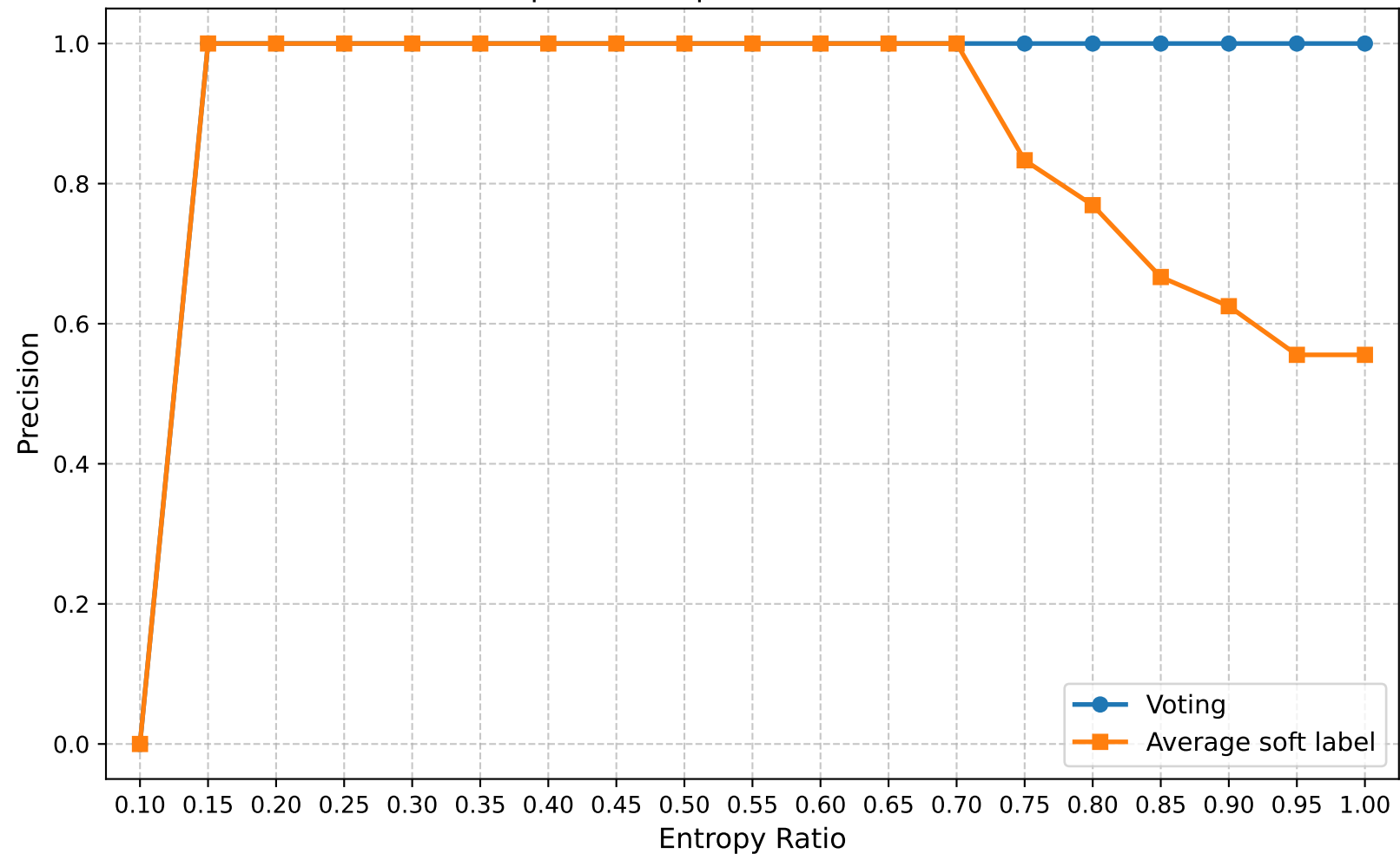
Precision | Round 5 | Confuse Model Ratio 0.30
