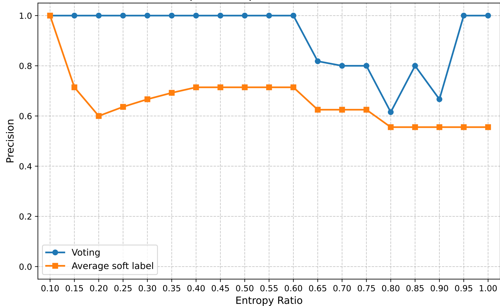
Precision | Round 5 | Confuse Model Ratio 0.70
