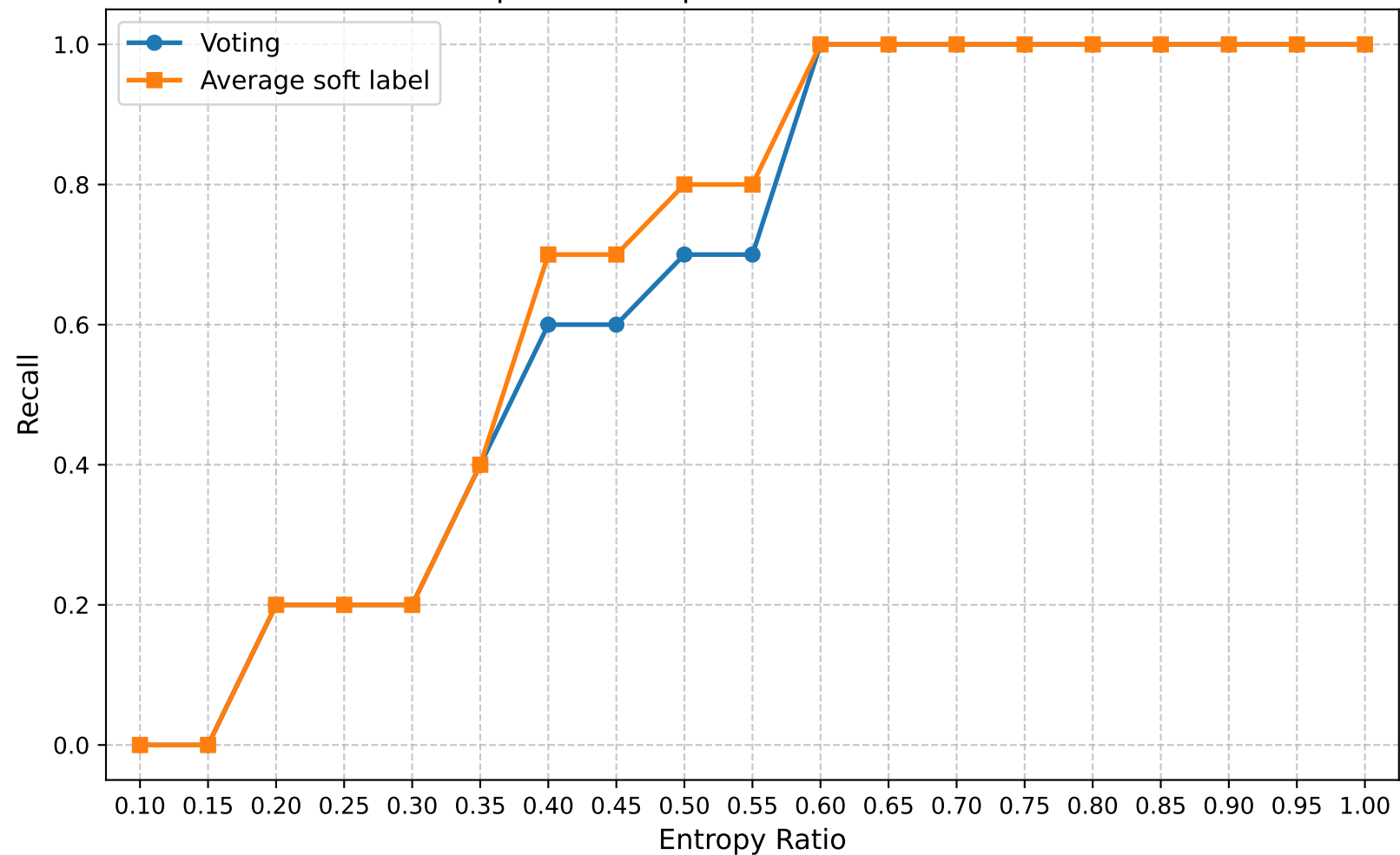
Recall | Round 10 | Confuse Model Ratio 0.30
