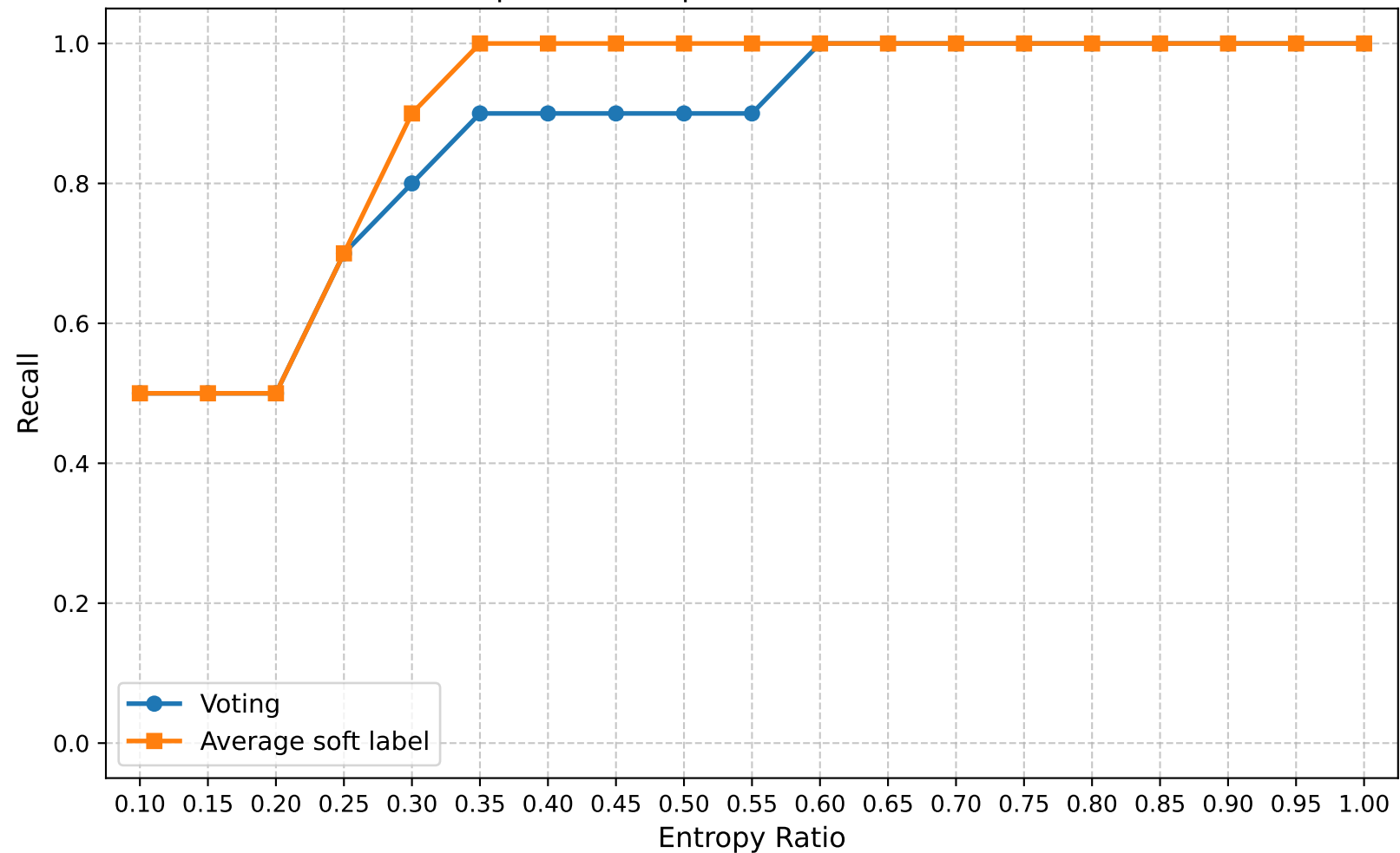
Recall | Round 10 | Confuse Model Ratio 0.80
