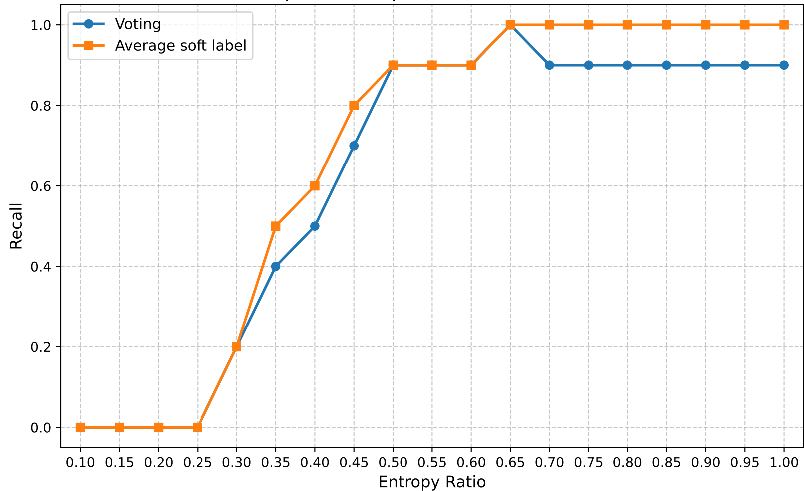
Recall | Round 15 | Confuse Model Ratio 0.30
