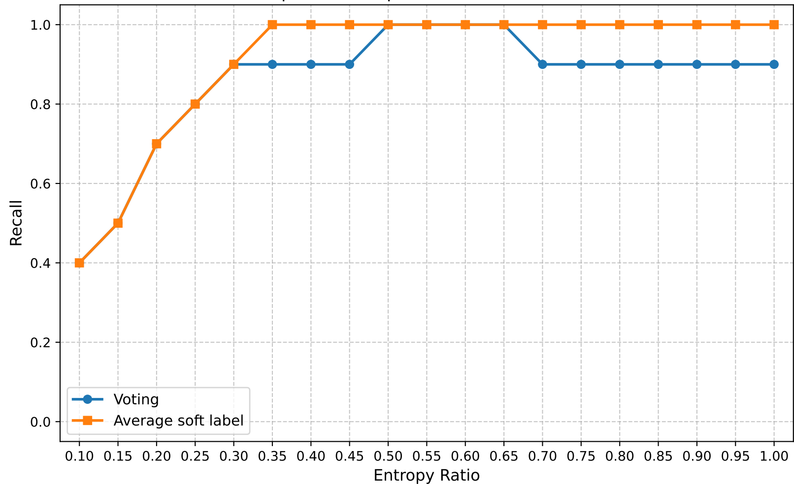
Recall | Round 15 | Confuse Model Ratio 1.00
