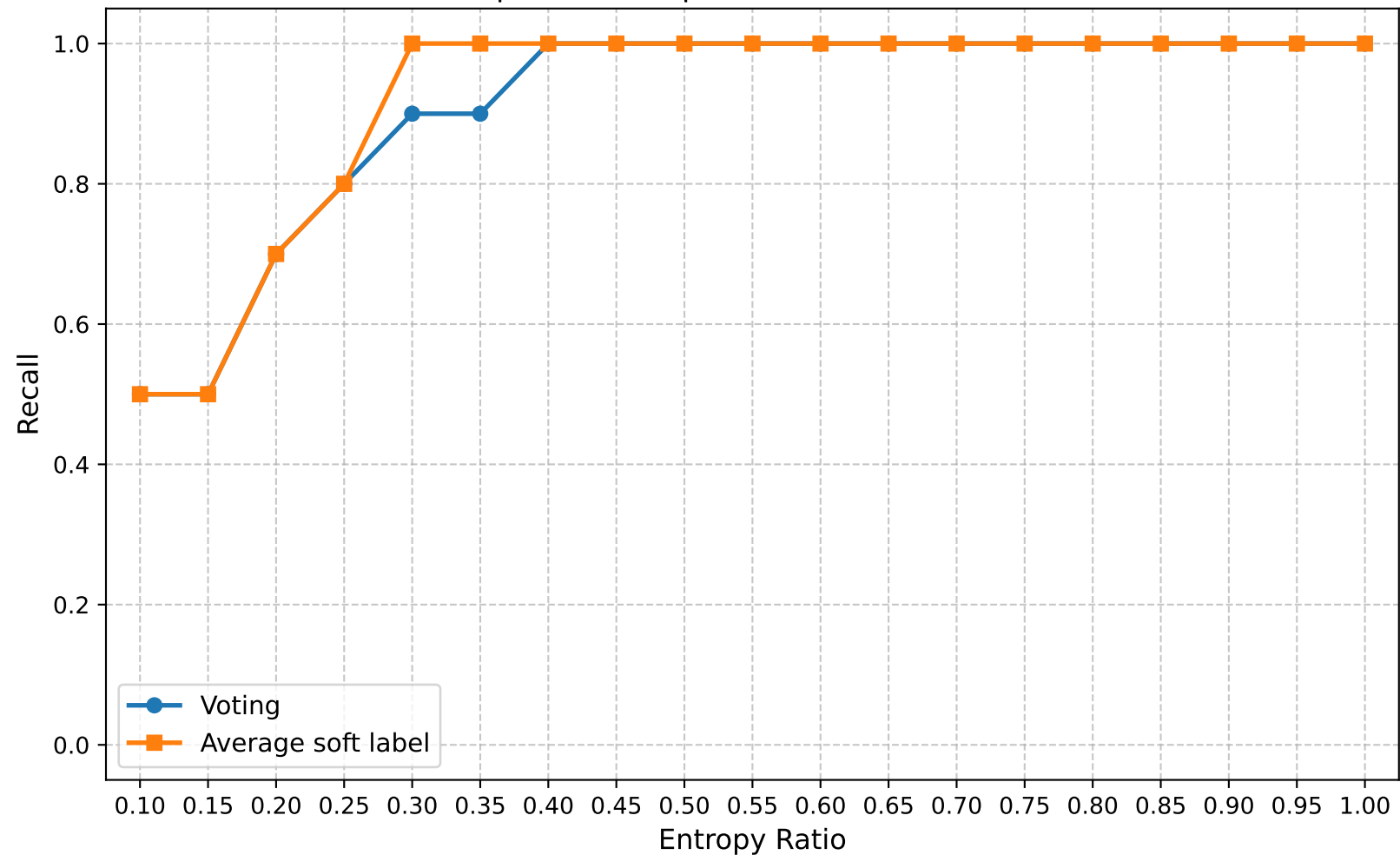
Recall | Round 25 | Confuse Model Ratio 1.00
