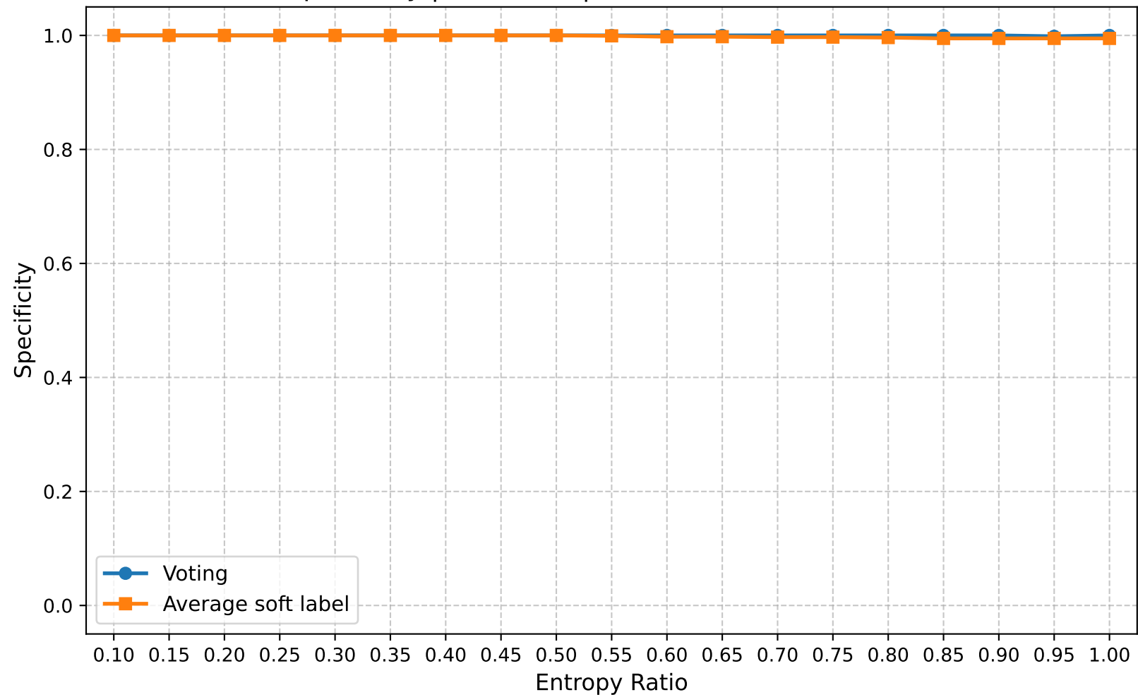
Specificity | Round 20 | Confuse Model Ratio 0.50
