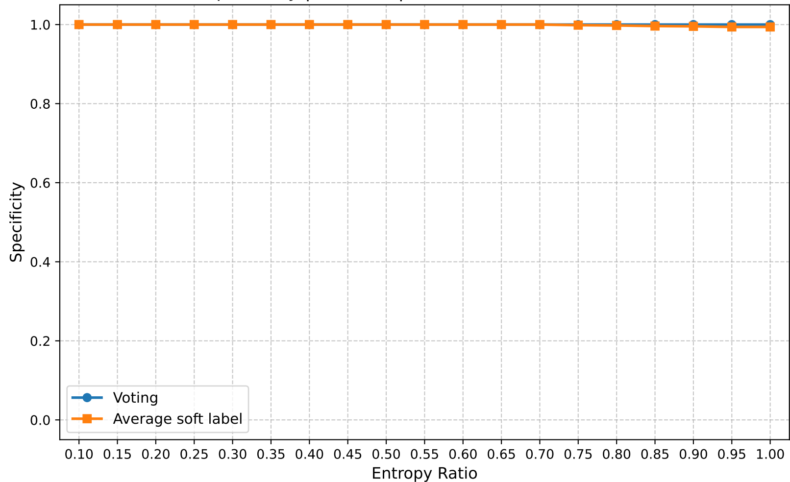
Specificity | Round 5 | Confuse Model Ratio 0.30
