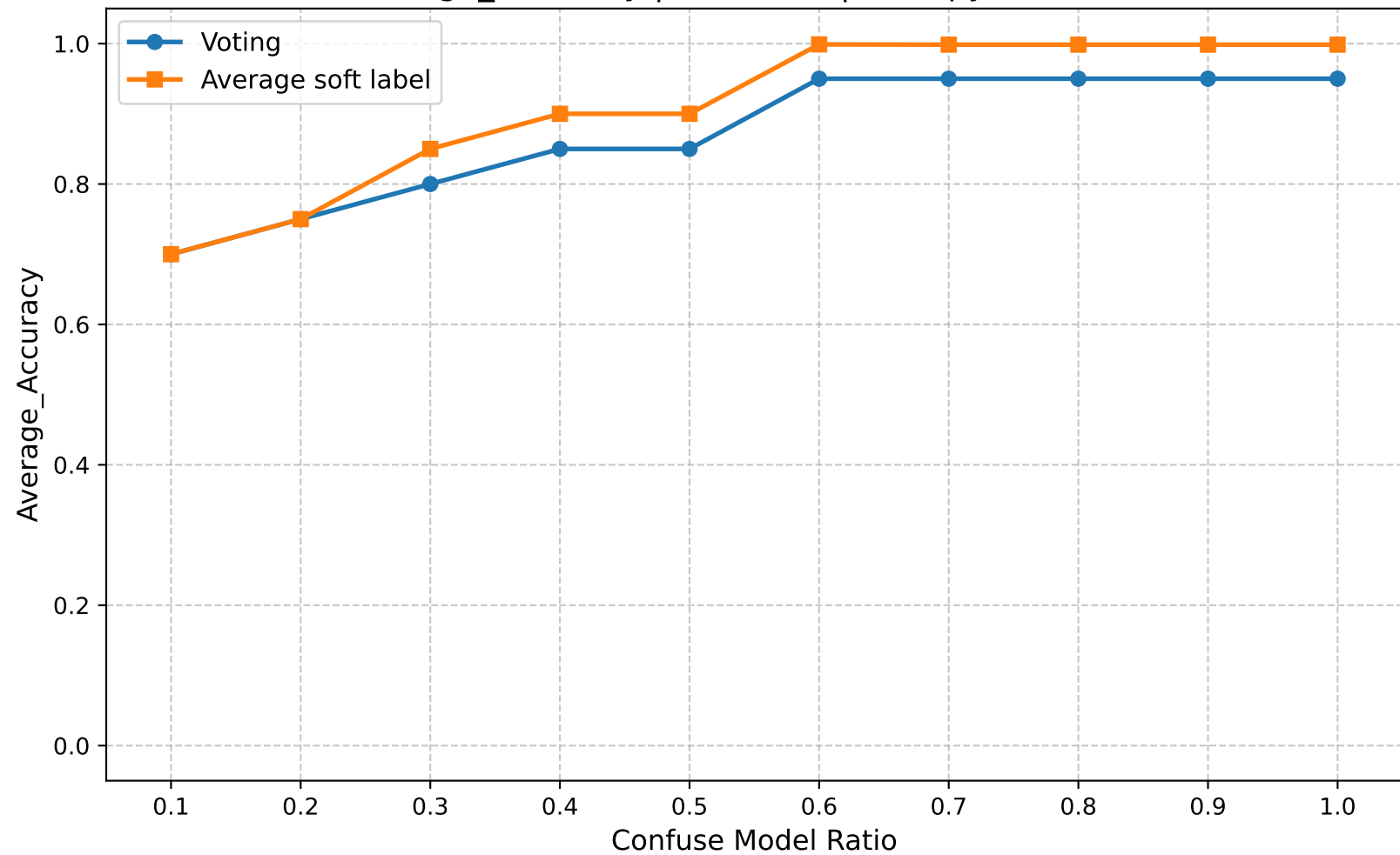
Average_Accuracy | Round 10 | Entropy Ratio 0.40
