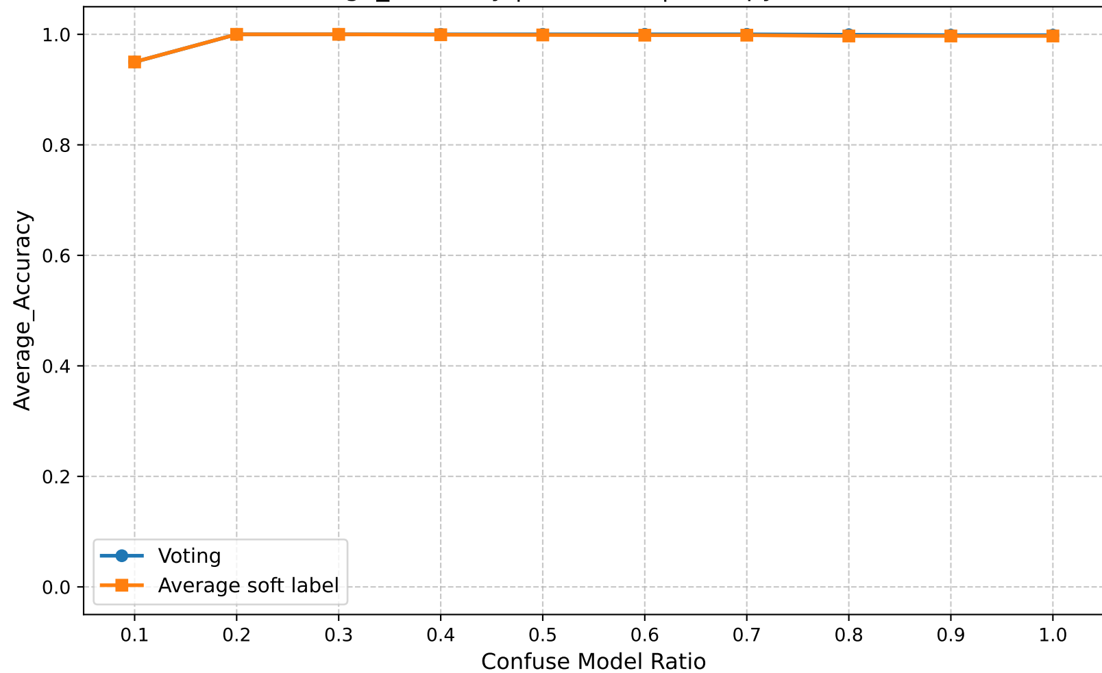
Average_Accuracy | Round 10 | Entropy Ratio 0.65
