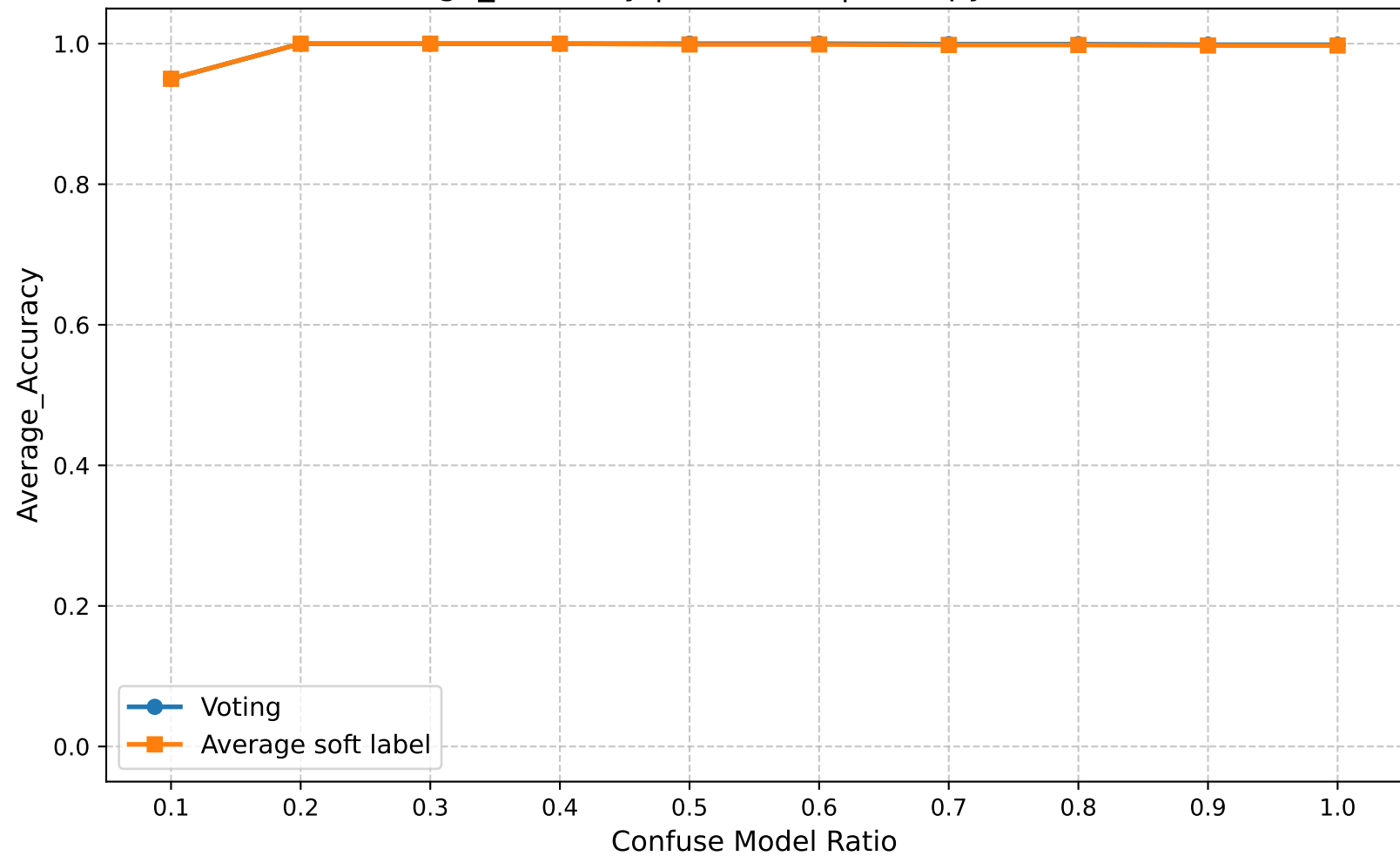
Average_Accuracy | Round 15 | Entropy Ratio 0.65
