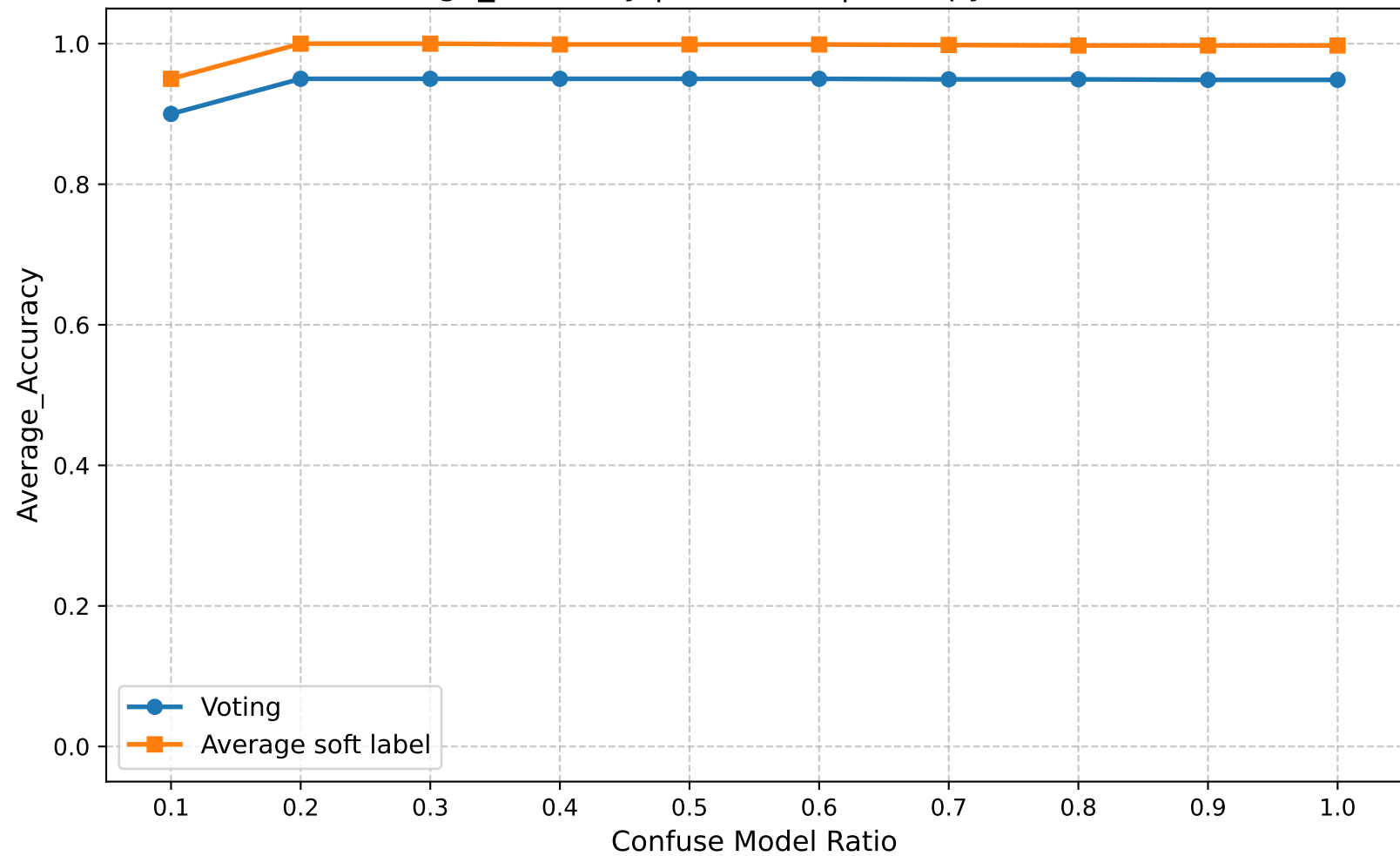
Average_Accuracy | Round 15 | Entropy Ratio 0.70
