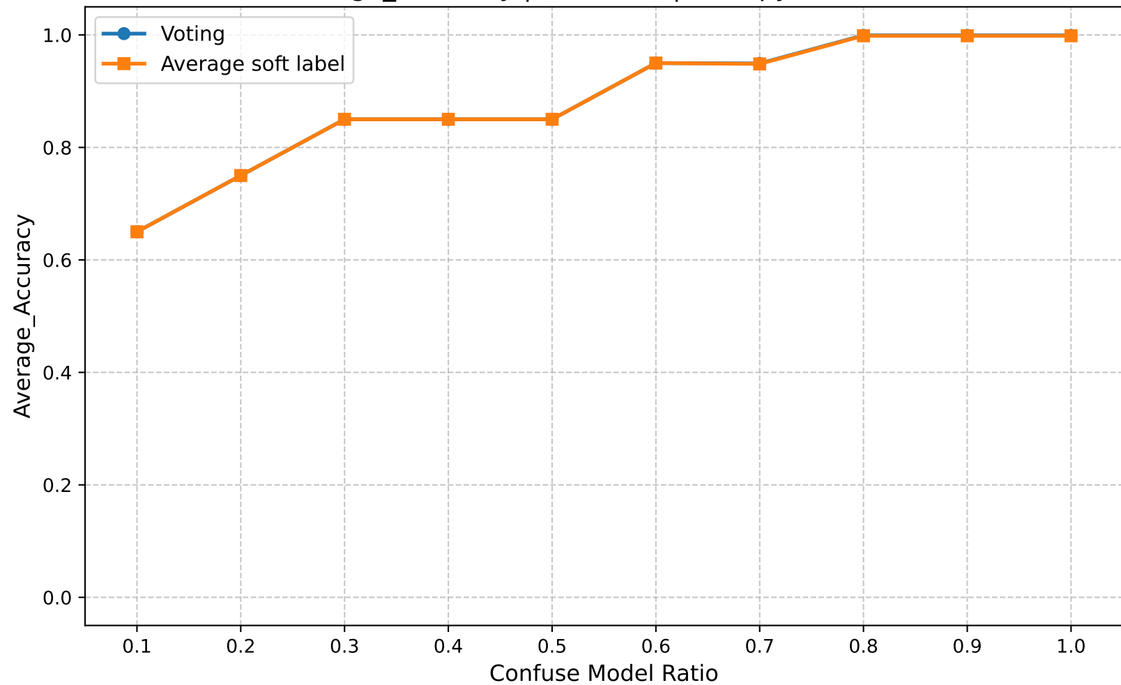
Average_Accuracy | Round 20 | Entropy Ratio 0.40
