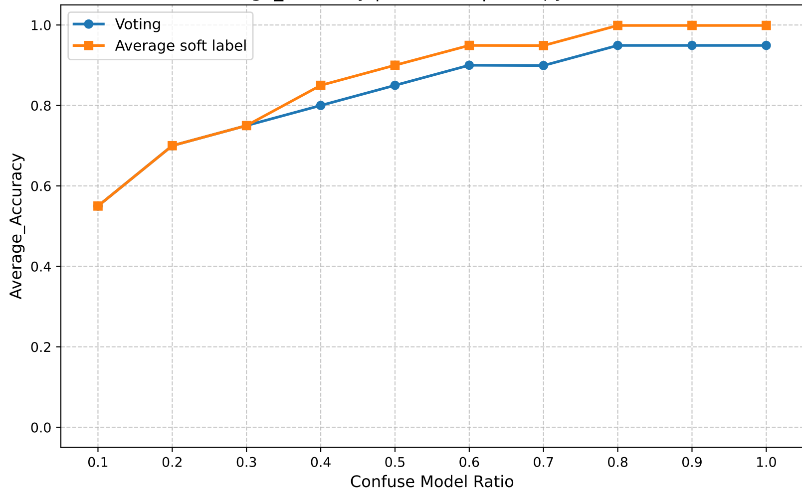
Average_Accuracy | Round 25 | Entropy Ratio 0.35
