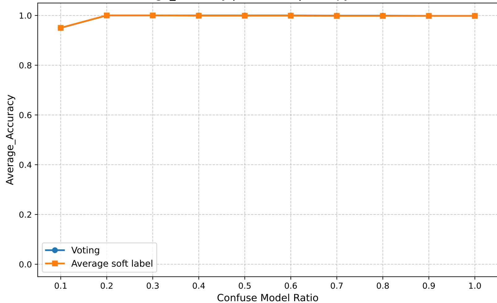
Average_Accuracy | Round 25 | Entropy Ratio 0.70
