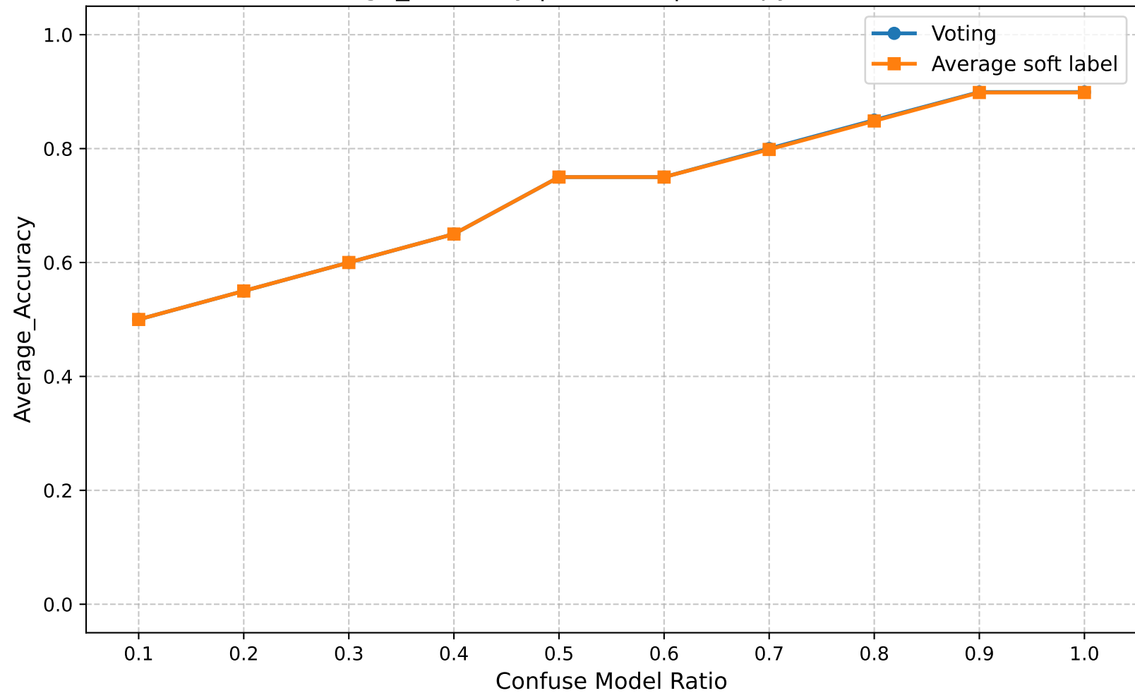
Average_Accuracy | Round 5 | Entropy Ratio 0.20
