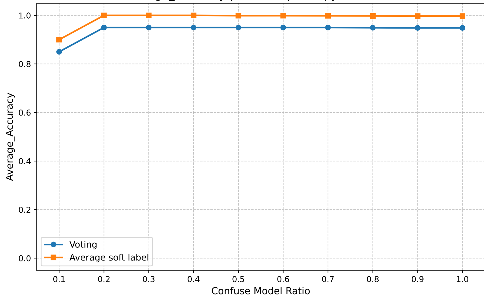
Average_Accuracy | Round 5 | Entropy Ratio 0.60
