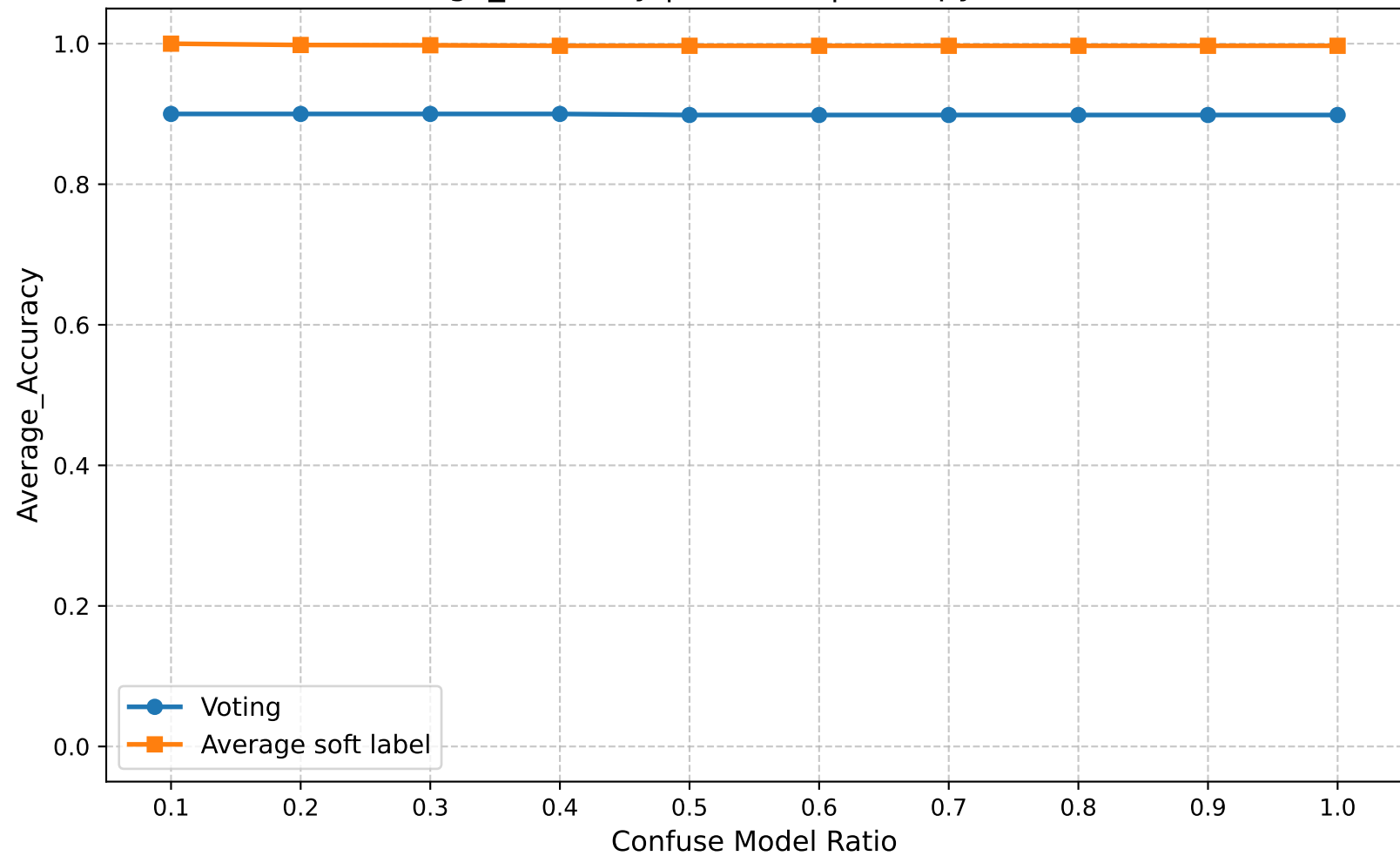
Average_Accuracy | Round 5 | Entropy Ratio 0.90
